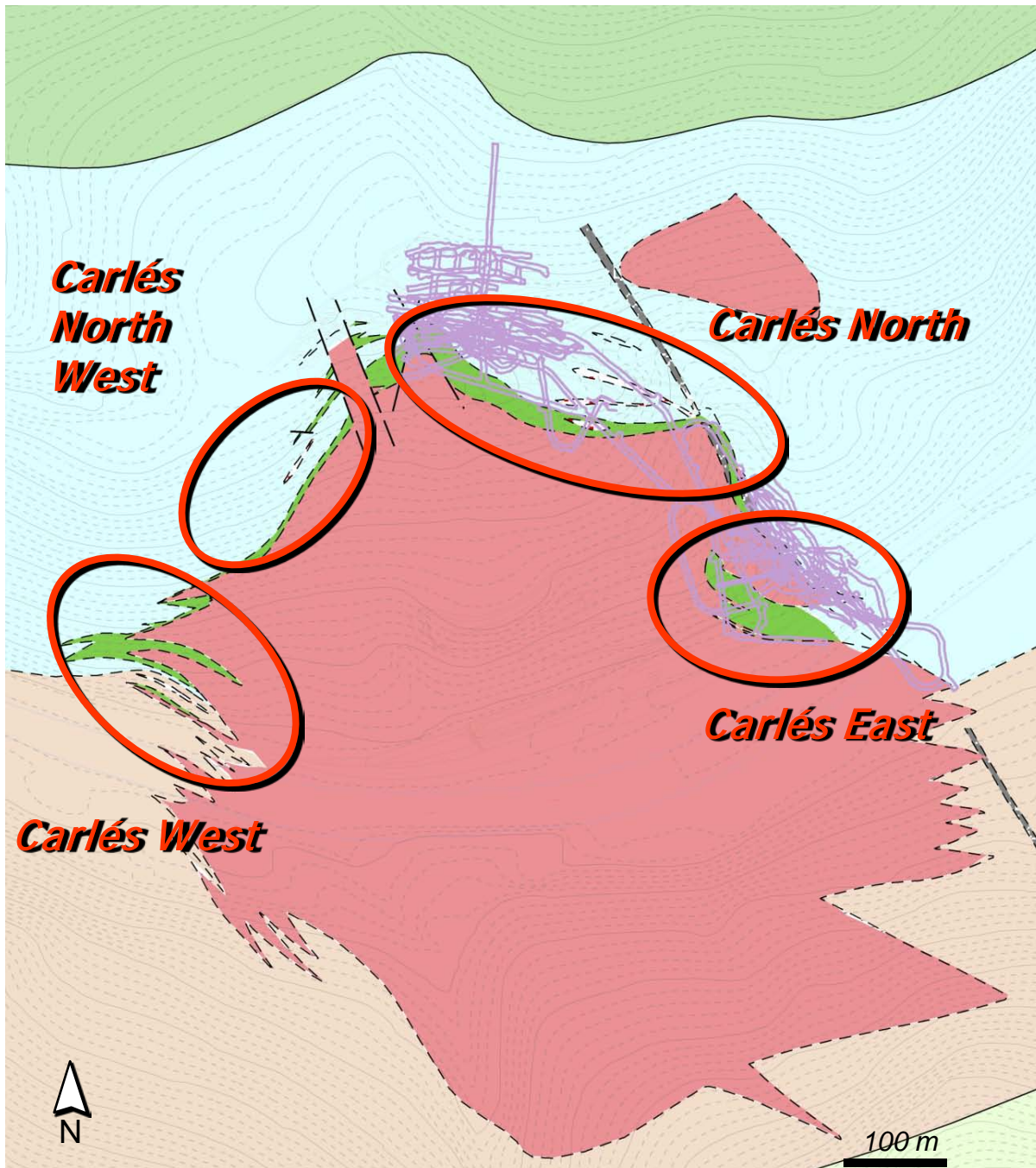
Location of the Carlés Mineralized Zones
